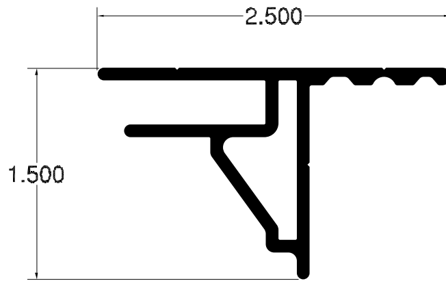
Flat Bleed Rigid Retainer Part# 2204
